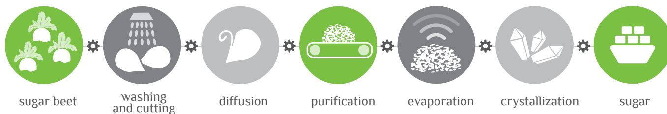
Stages of white sugar production
